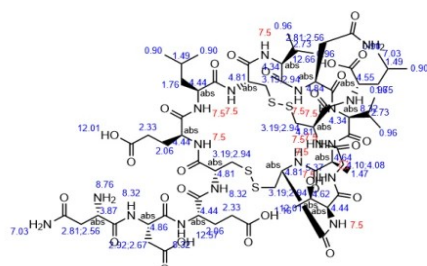
ChemNMR 1 H Estimation
